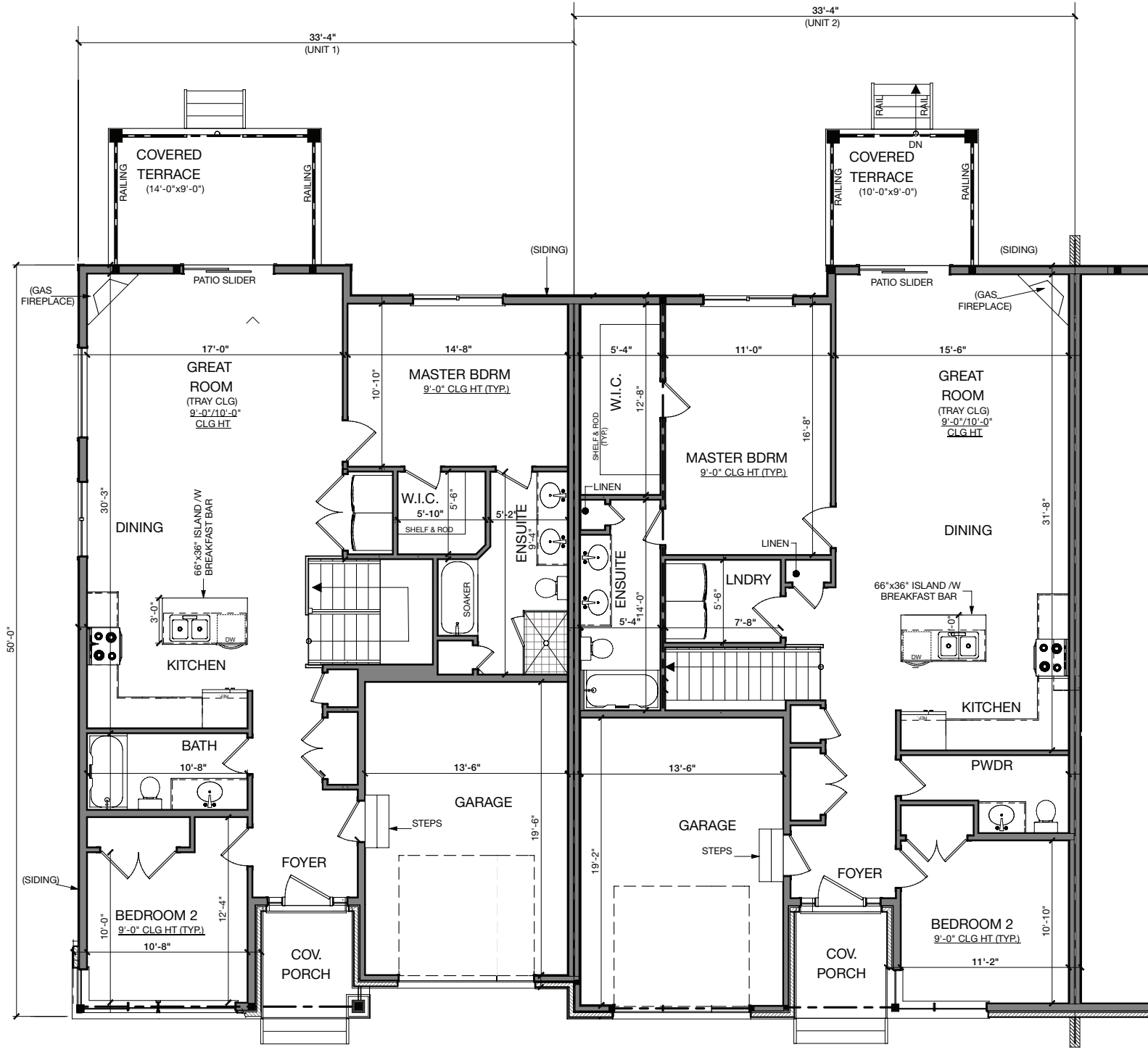
UNIT #1 MAIN FLOOR - 1,264 SQ. FT
