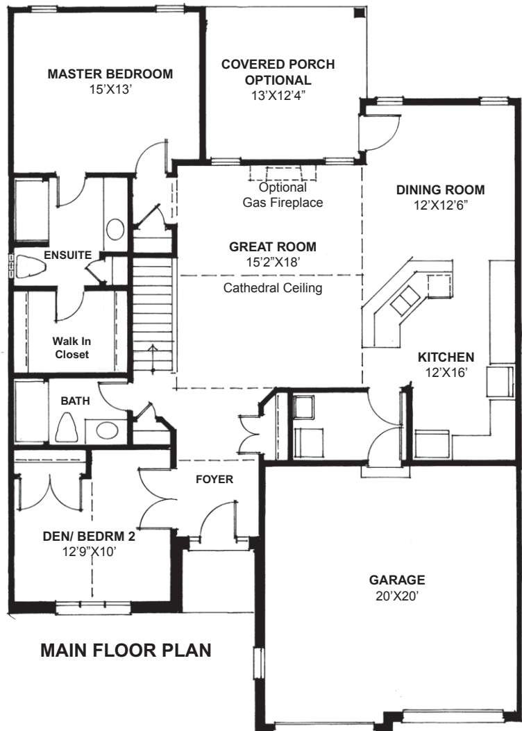
Plans as drawn show approximate only, and actual sizes, specifications, cabinetry and square footage of the completed dwelling may vary slightly.
